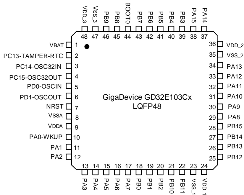
Figure 2-4. GD32E103Cx LQFP48 pinouts
